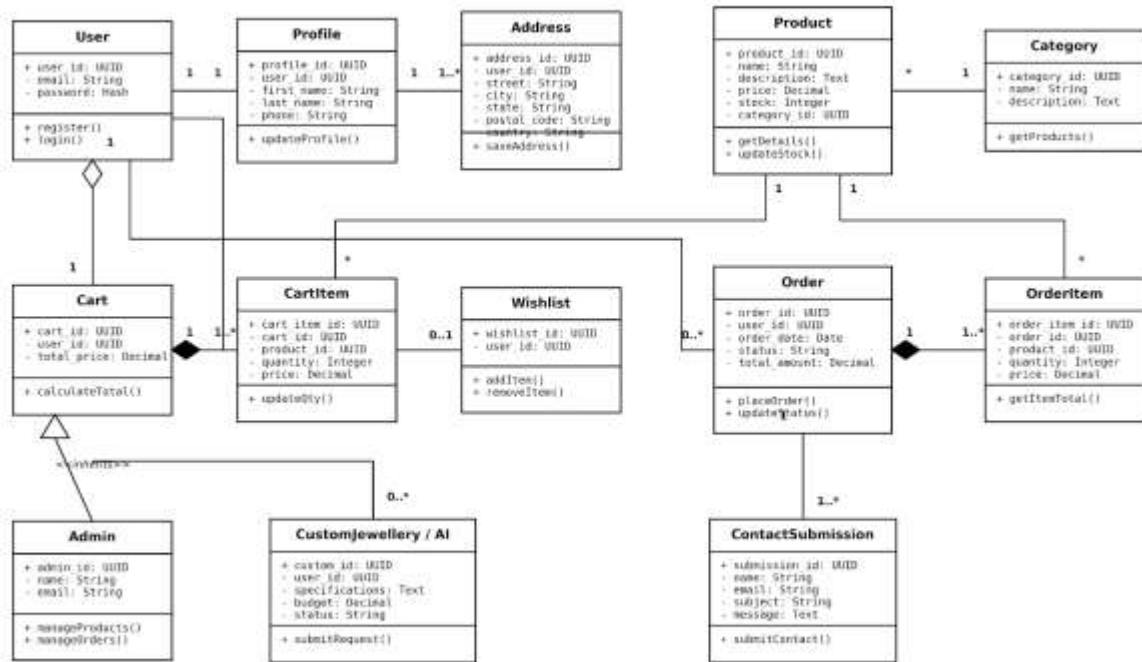
Figure 3: MEERA Class Diagram
