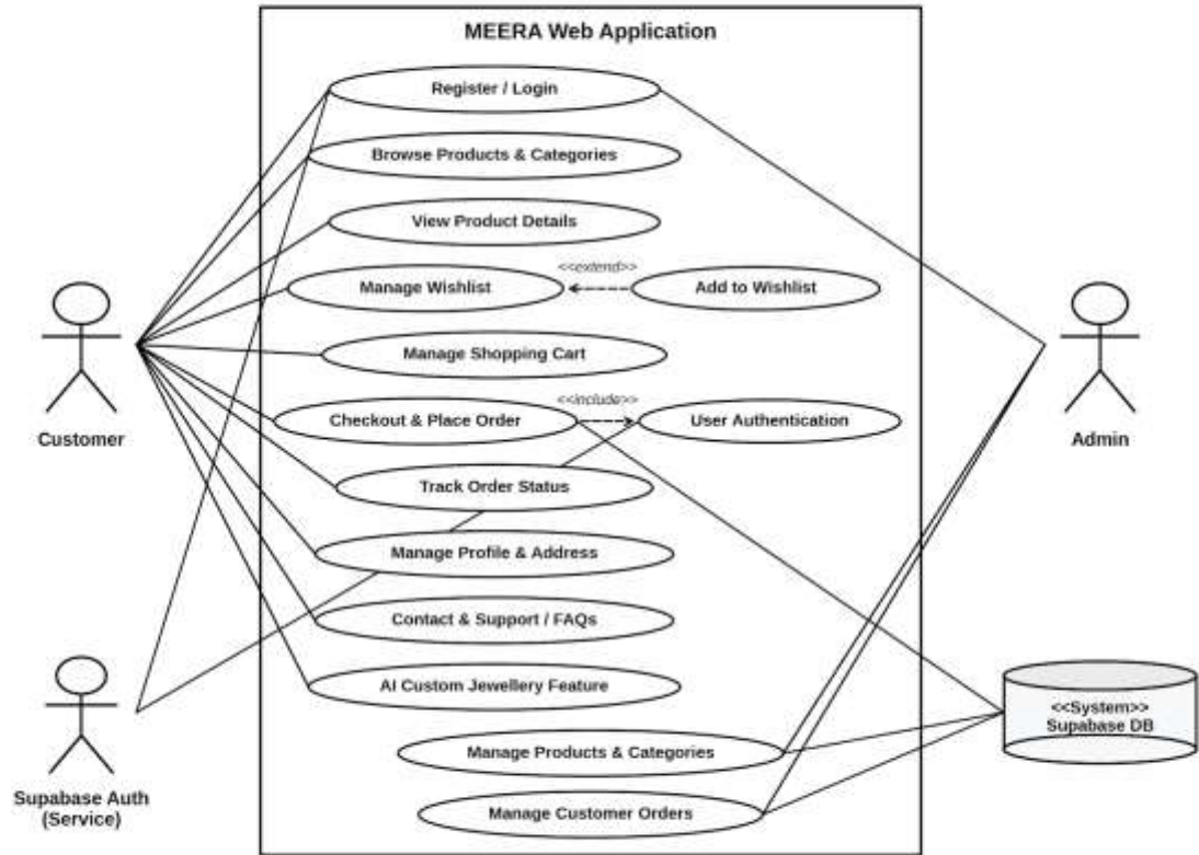
Figure 1: MEERA Use Case Diagram
