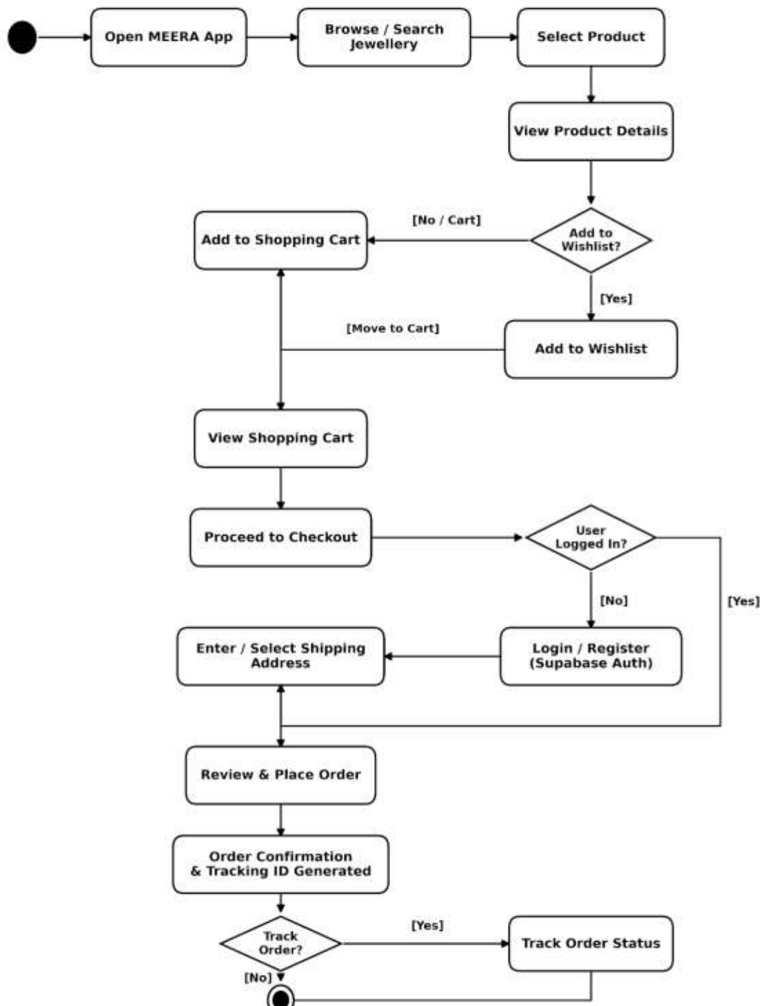
Figure 2: MEERA Activity Diagram
